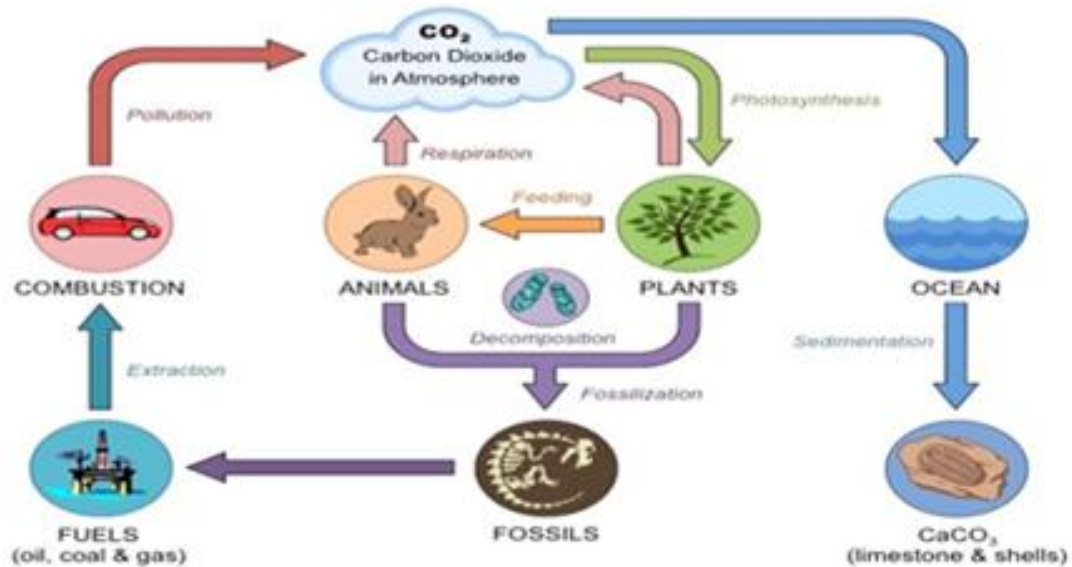
FIG.7.5: Carbon Cycle in Nature
